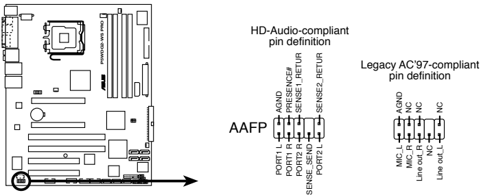
P5WDG2-WS PRO Front panel audio connector
