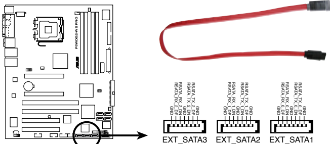
P5WDG2-WS PRO SATA 3 Gbps connector
