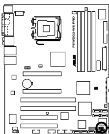
P5WDG2-WS PRO Clear RTC RAM
