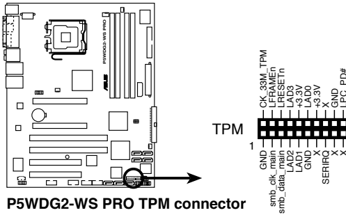
P5WDG2-WS PRO TPM connector
