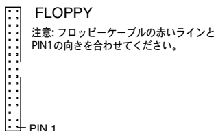
P5WDG2-WS PRO Floppy disk drive connector
